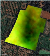
RVI (For Crop Health)
