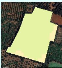
DEM (For Flood Analysis)
