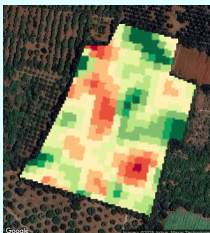
RSM (For Irrigation)
