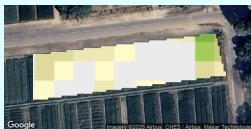
NDWI Image (For Irrigation)
