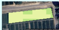
SOC (For Soil Carbon Analysis)
